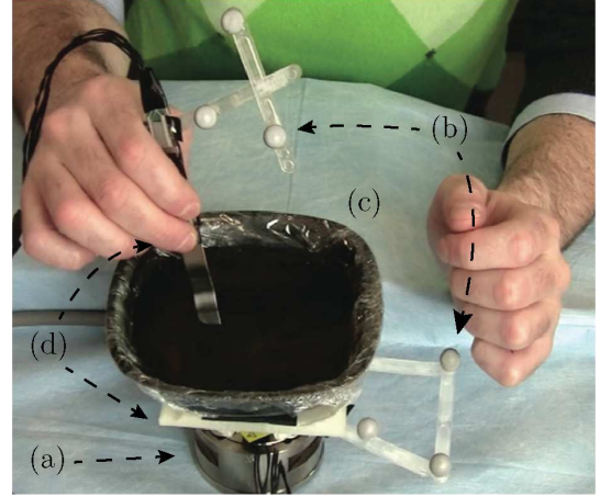
Figure 3: Setup for interaction forces acquisition. The surgeon is performing the cut test with spatula (SpK). The (a) multi-axis load cell, the (b) passive optical markers on the tool and on the ABS plate base, and (c) the brain phantom are visible, whereas the (d) ABS plate and the contact force sensors are partially occluded.
